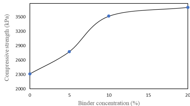
Fig. 2. A plot of compressive strength (kPa) versus binder concentration (%).
