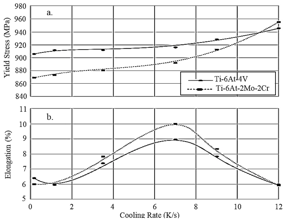
Fig. 8a-8b. Yield stress and tensile elongation dependence on the cooling rate from \beta -phase range for selected titanium alloys.
