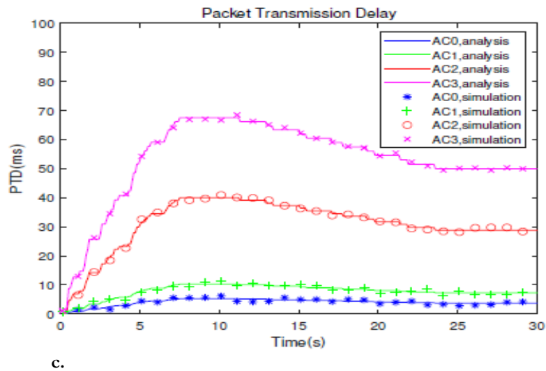
Fig. 4. The packet transmission delay that is time dependent. A left turn, a straight shot, or a right turn, respectively [3].
