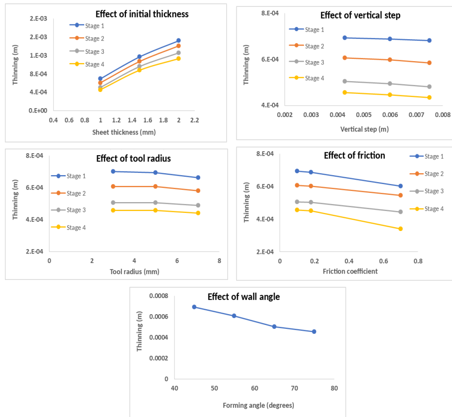
Fig. 11. Effect of the parameters of the sheet thickness, the tool radius, the wall angle, the vertical step and the friction coefficient on the critical thickness.
