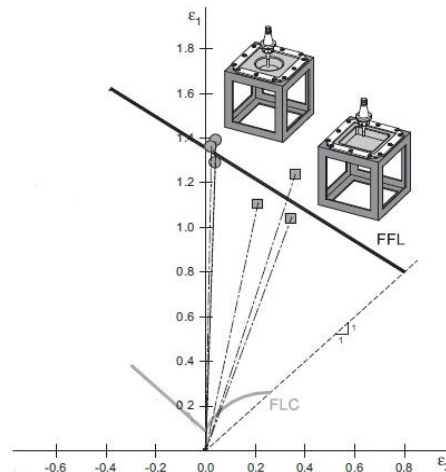
Fig. 2. Schematic of the location of the principal strains in the regions close to the crack in the cone and the pyramid [40].
