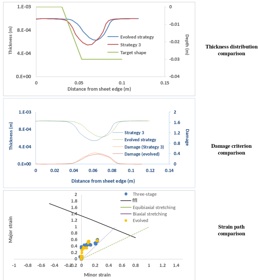
Fig. 10. Combined diagram of the comparison of the thickness, the damage criterion and the strain path in the three-stage and the evolved strategies.
