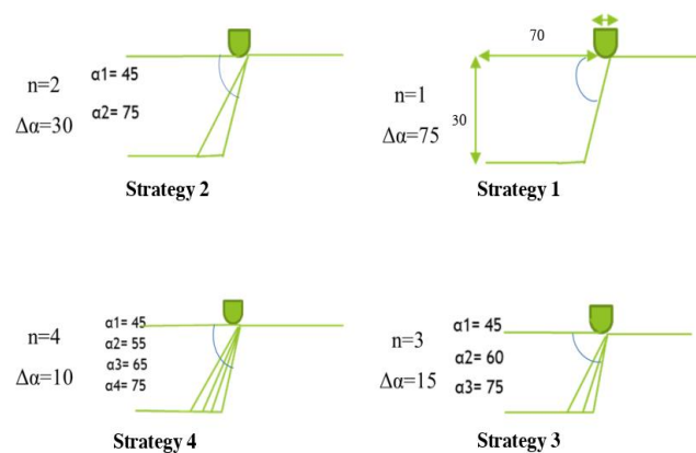
Fig. 6. Combined schematic of the single-stage, two-, three- and four-stage strategies.
