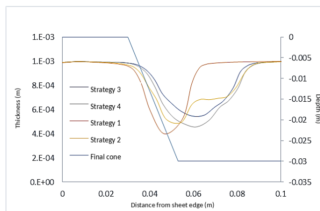
Fig. 7. Comparison of the final thickness distribution in the one-, two-, three- and four-stage strategies.
