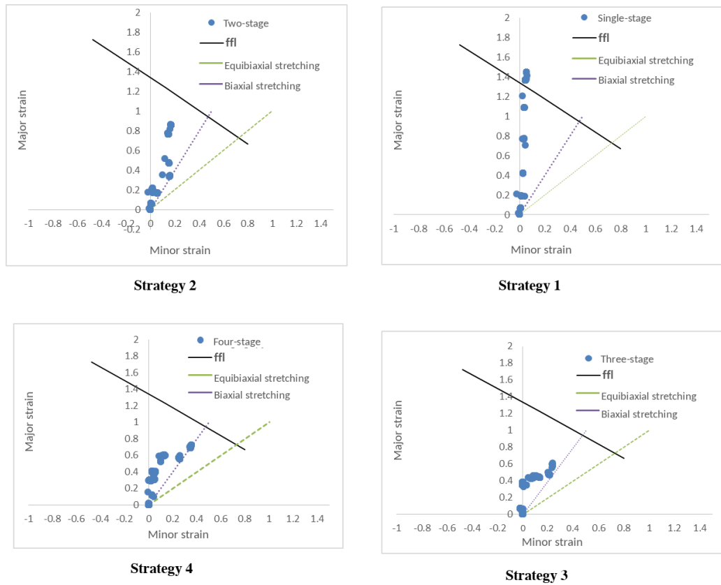
Fig. 8. Combined diagram of the strain path of the single-stage, two-, three- and four-stage processes with respect to the FFLD line.
