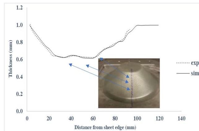
Fig. 5. Comparison of the thickness distribution obtained from the experimental results and from the simulation.
