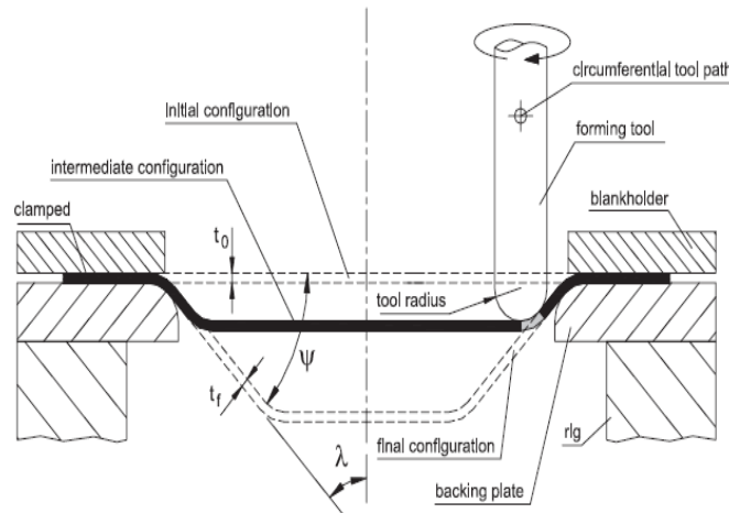
Fig. 1. Representation of the rotationally symmetric single point incremental forming process SPIF [11].
