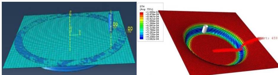
Fig. 3. Simulation of the single point incremental forming process in Abaqus software.
